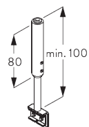
SG 3610 Suspension
