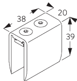
SG 6610 Support mural
