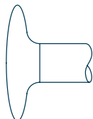
Ellipse
